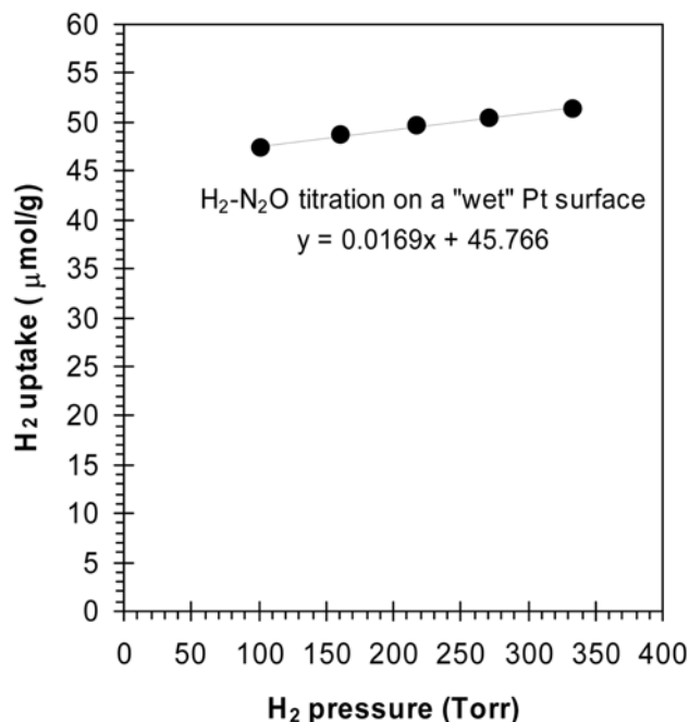
Fig. 8. An adsorption isotherm for \text{H}_2 adsorption at 300 K on 0.65% Pt/SiO 2 after continuous \text{N}_2\text{O} reduction at 363 K in the presence of \text{H}_2 for 4 h following dissociative \text{N}_2\text{O} adsorption at 363 K.
