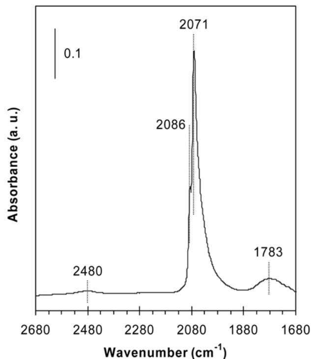
Fig. 9. In situ DRIFTS spectra of CO adsorbed at 300 K on 0.65% Pt/SiO 2 after continuous \text{N}_2\text{O} reduction at 363 K in the presence of \text{H}_2 for 4 h following dissociative \text{N}_2\text{O} adsorption and subsequent \text{H}_2 adsorption at 363 K. This spectrum was recorded after a 30-min purge with He at 300 K.
